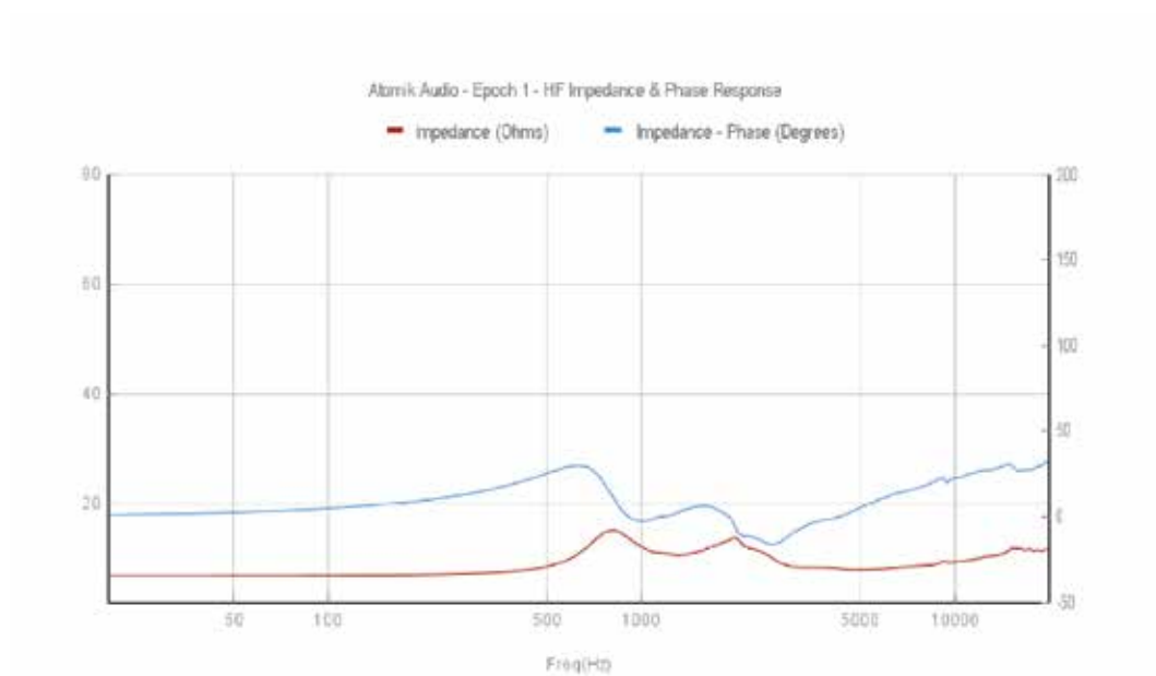
HF Impedance & Phase Response
